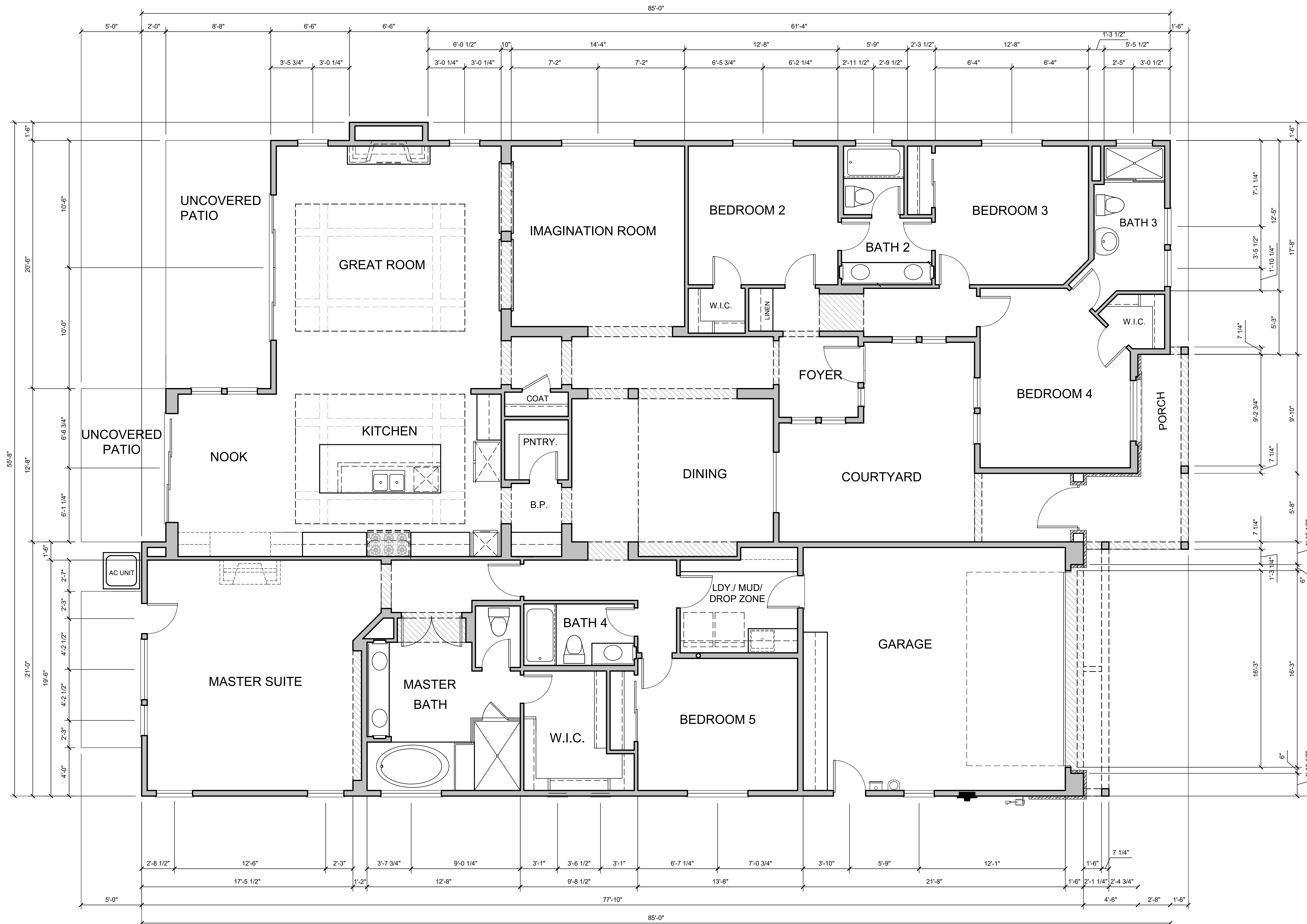
PLAN 5, LOT 5 FLOOR PLAN
